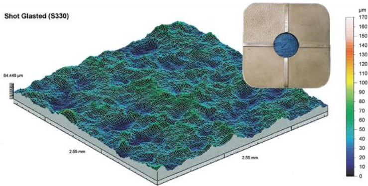
Figure 2. Surface Profile for shot blasted surfaces.
