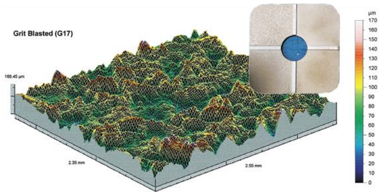
Figure 3. Surface Profile for grit blasted surfaces.
